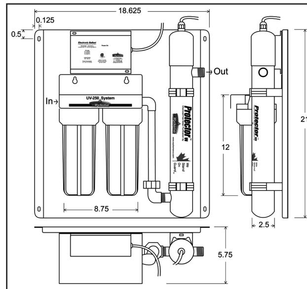
SYS250-POU Dimensional. All measurements in inches
